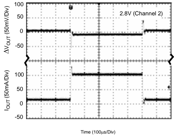
Figure 39. Load Transient
