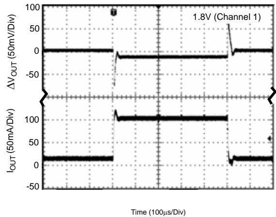
Figure 37. Load Transient
