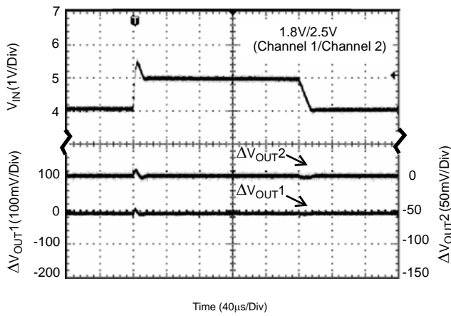
Figure 36. Line Transient
